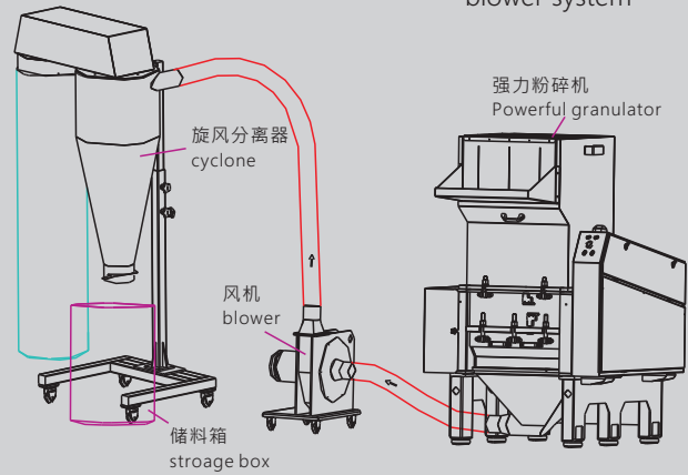
Powerful granulator Installation diagram ----blower system
