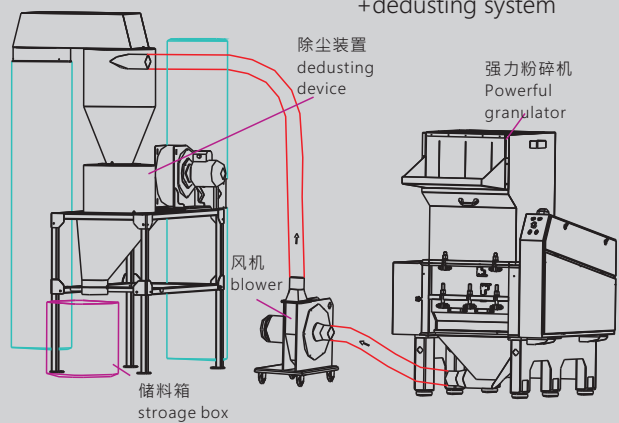
Powerful granulator Installation diagram --blower system +dedusting system
