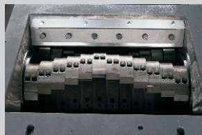
RG-56EA 爪刀型 Staggered blades type
