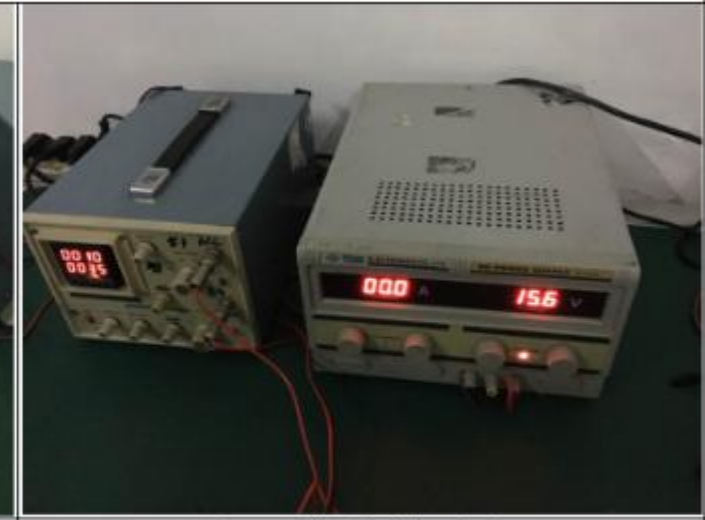
Power fluctuation test Keep Voltage 15.6V,the machine make Android units power turn on and turn off automotively. The steps repeat again and again.
