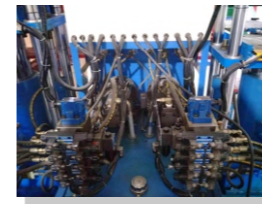
双独立运作马达 Two independent motor
