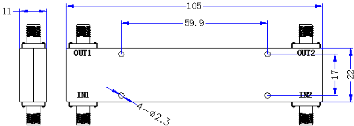
Figure 1 JX-BC3-700M2700M-20S front panel layout
