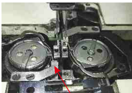
直刀剪线结构 Straight knife cut line structure
