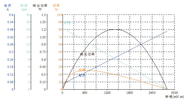
Model: DM-22RPL1800249000-509K
