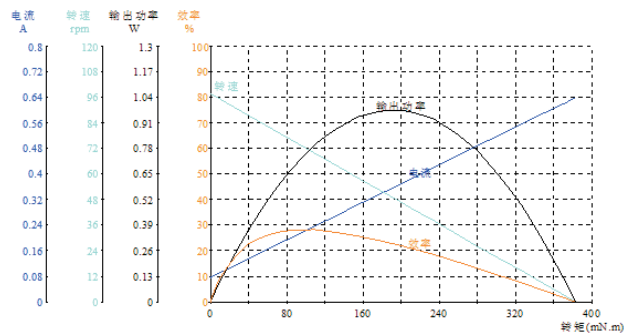
Model: DM-22RPL1800127000-64K
