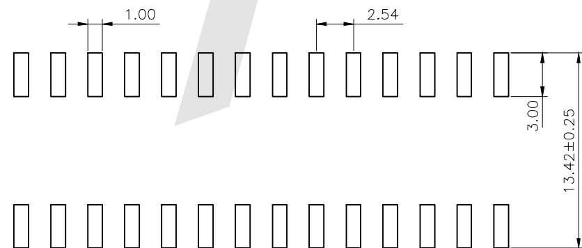
PCB LAYOUT
