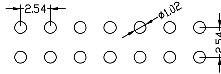
PCB LAYOUT
