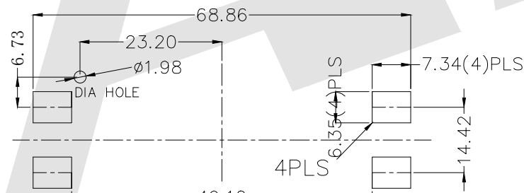
MOUNTING PAD LAYOUT
