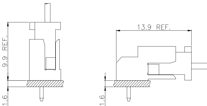
DIP TYPE
