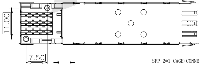
SFP 2*1 CAGE+CONNECTOR
