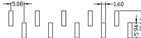
TYPE A PCB LAYOUT
