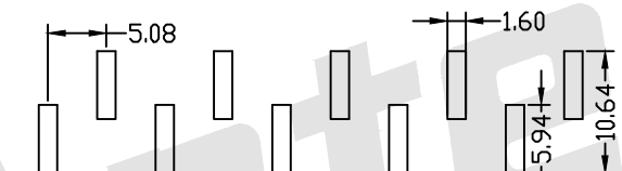
TYPE B PCB LAYOUT
