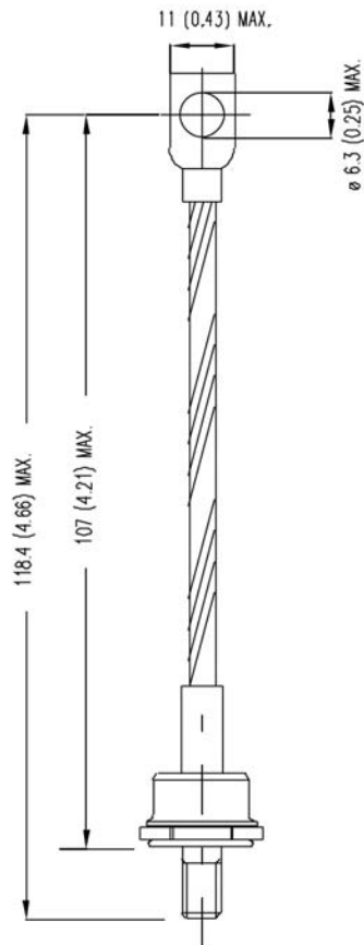
41HF(R) Case Style DO-203AB (DO-5) All dimensions in millimeters (inches)
