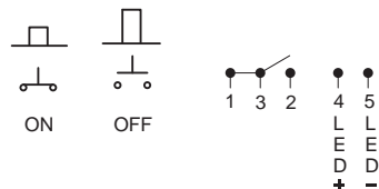
CIRCUIT
