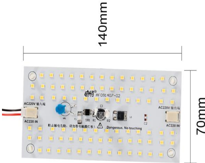
9W LED module entity diagram
