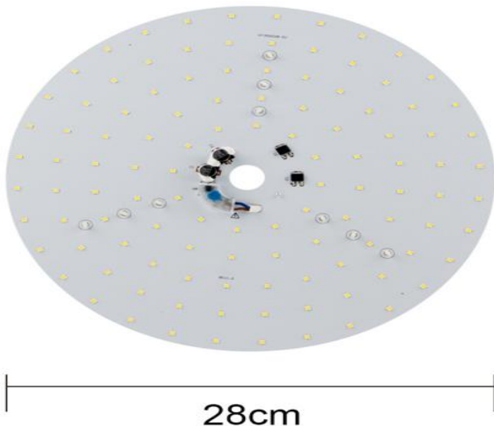
35W LED module entity diagram
