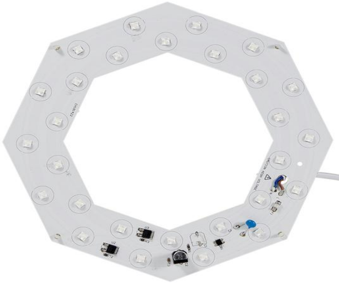
26W LED module entity diagram
