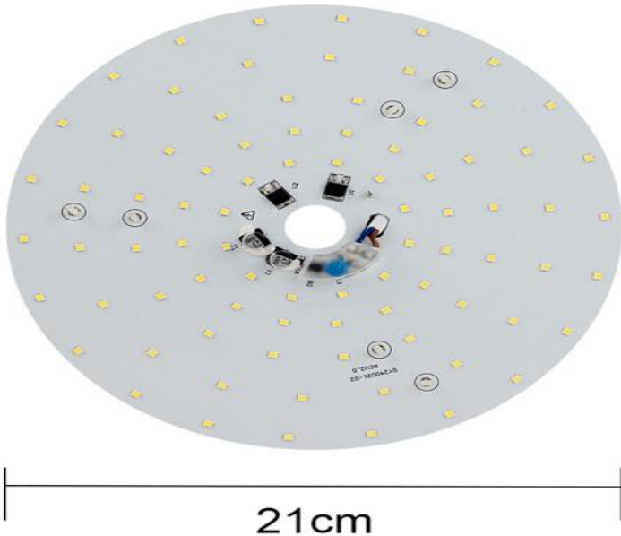
24W LED module entity diagram
