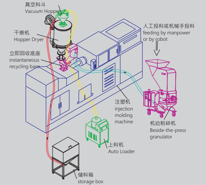
Beside-the-press granulator installation diagram ----Blower system
