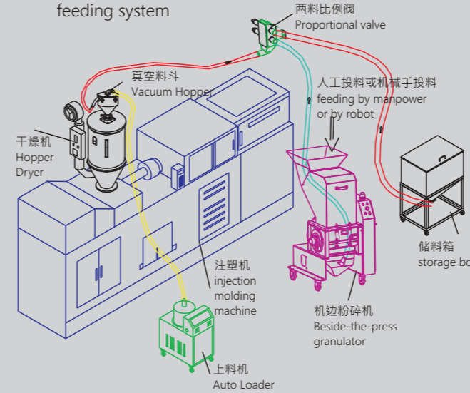
Beside-the-press granulator installation diagram ----Proportional valve feeding system
