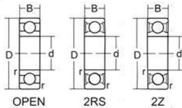
Deep Groove Ball Bearings of 6000 Series
