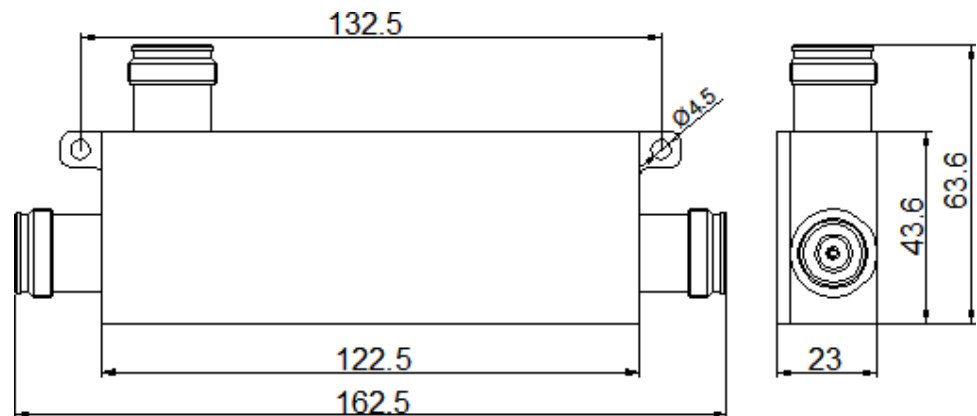
Figure 1 JX-PC-575-6000-XC43DI Coupler
