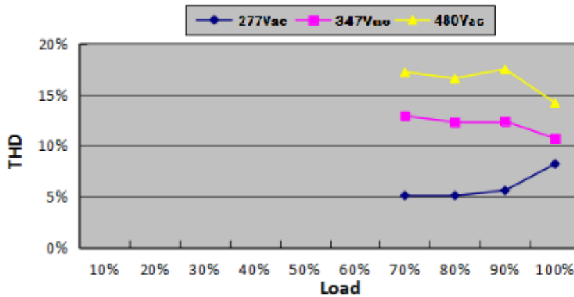
THD vs. Load Curve
