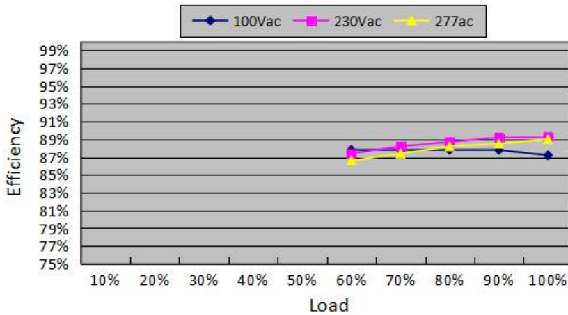
Efficiency vs. Load Curve
