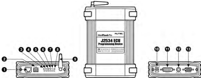
Figure 2-4 J2534 ECU Programming Device
