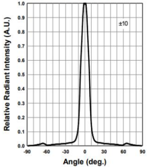
Radiation Characteristics
