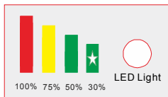
Battery Full/Output Setting by Light Color
