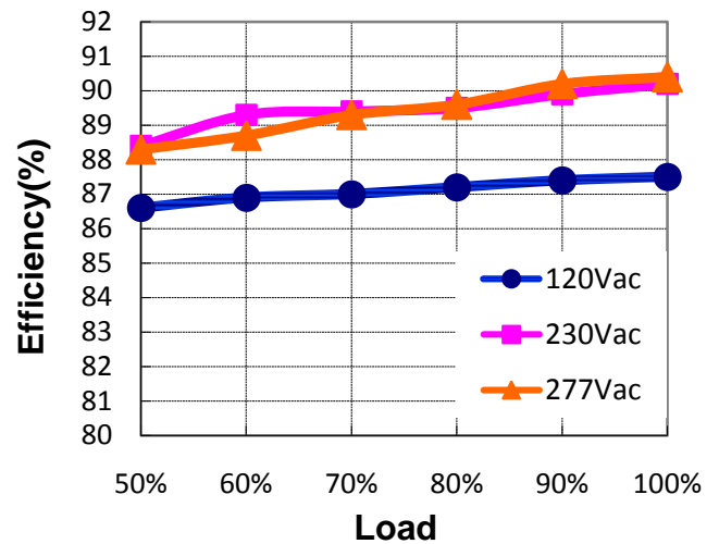
MTP-120X068(Io=1.77A) Efficiency VS Load
