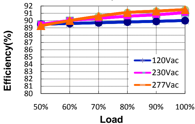
MTP-120X068(Io=2.15A) Efficiency VS Load
