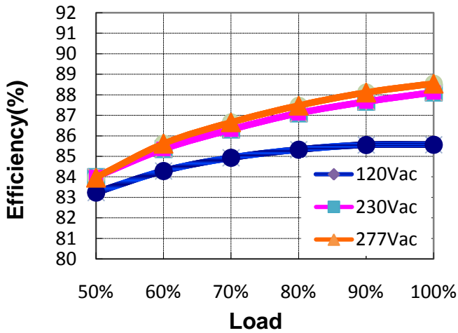
MTP-120X040(Io=3.75A) Efficiency VS Load
