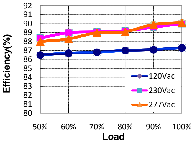
MTP-120X068(Io=2.15A) Efficiency VS Load
