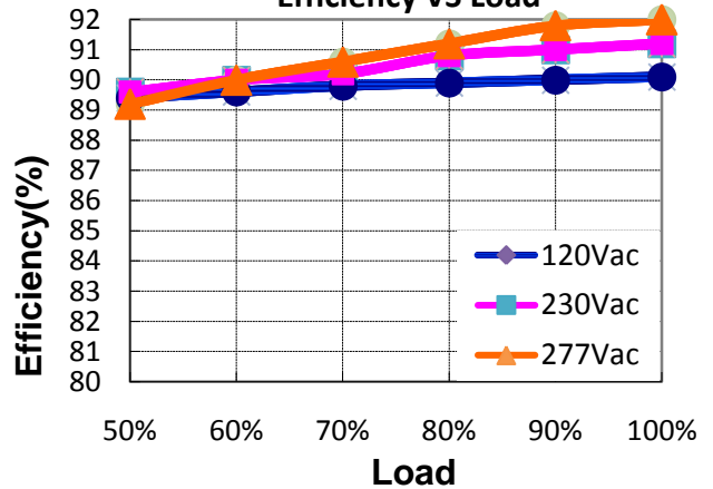
MTP-120X068(Io=1.77A) Efficiency VS Load
