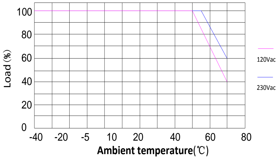
Derating curve
