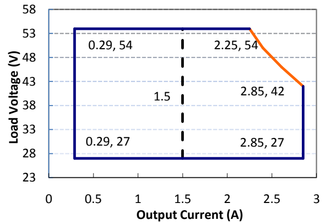
Output Current Vs Load Voltage Curve
