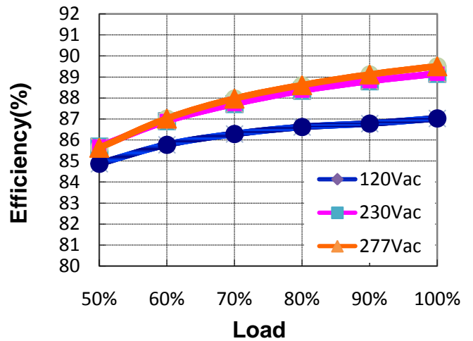
MTP-120X054(Io=2.25A) Efficiency VS Load
