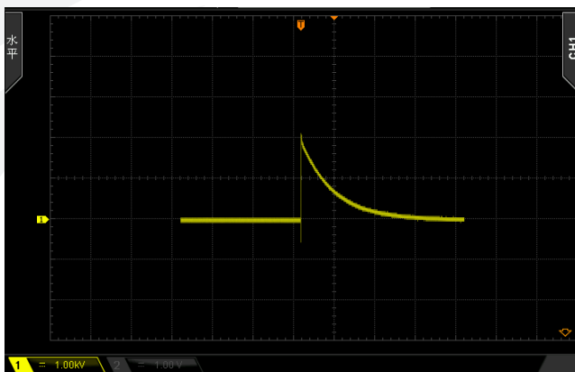
Input voltage waveform (differential mode 2KV)
