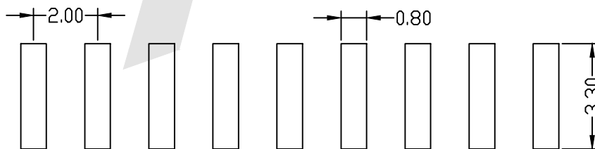
PCB LAYOUT
