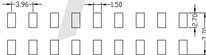
PCB LAYOUT
