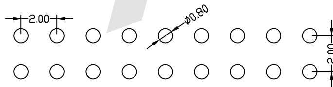
PCB LAYOUT
