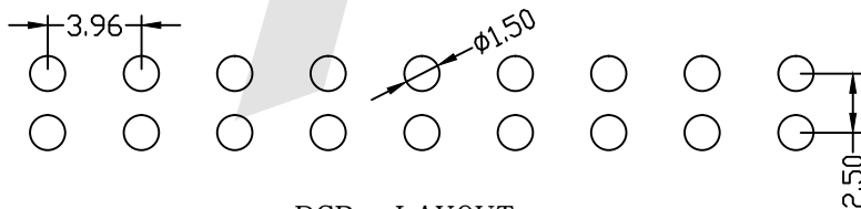
PCB LAYOUT
