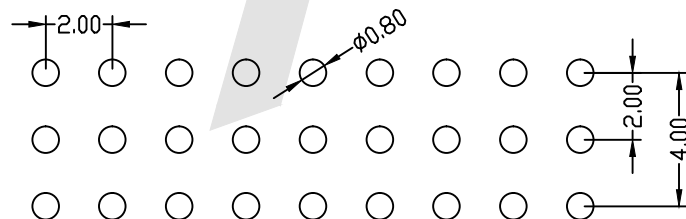
PCB LAYOUT
