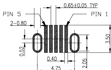
P.C.B LAYOUT (TOLERANCE:±0.05)
