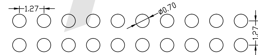
PCB LAYOUT
