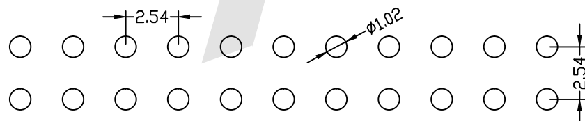
PCB LAYOUT
