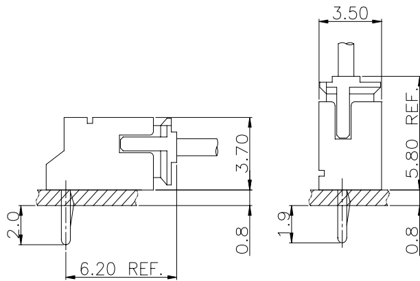
DIP TYPE
