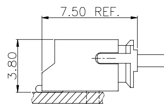
DIP TYPE
