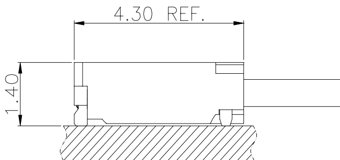
Right Angle Type
