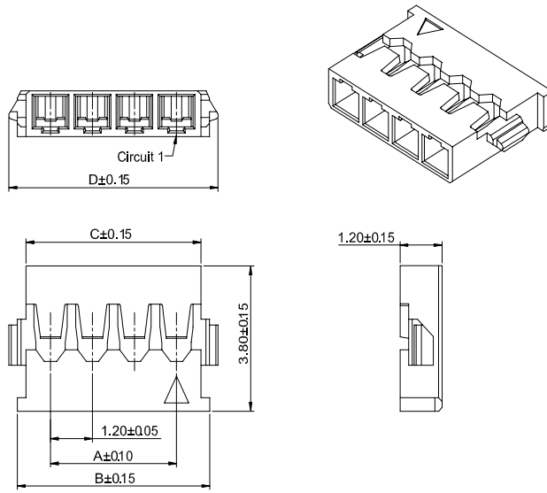
Ordering Information & Dimensions:
