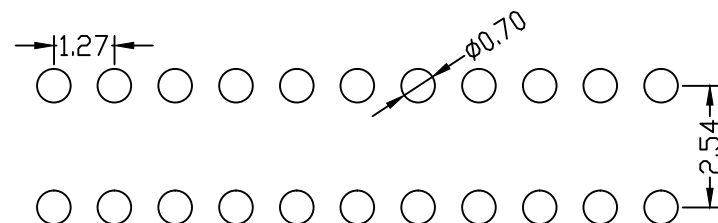
PCB LAYOUT
