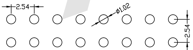
PCB LAYOUT
