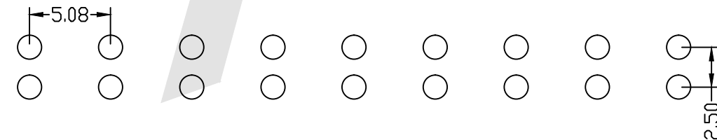
PCB LAYOUT
