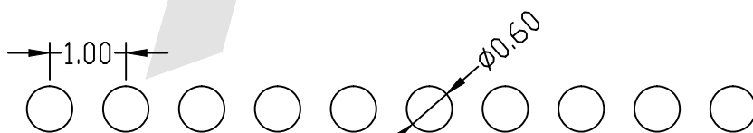
PCB LAYOUT
