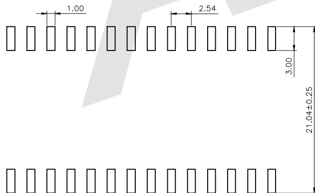
PCB LAYOUT
