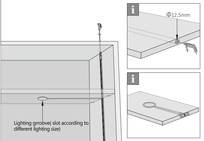
⑤ Open a hole \Phi 12.5\text{mm} on the side of Laminate, and put in power adaptor
