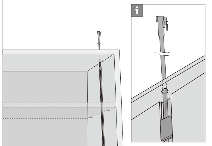
④ Connect input connector
