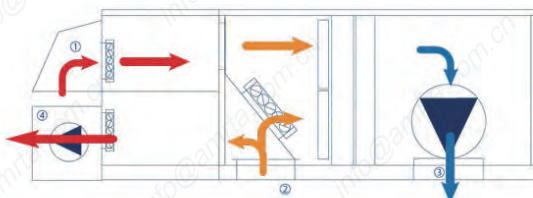
Cooling/heating mode with fresh air
