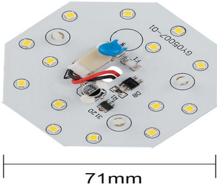
5W LED module entity diagram
